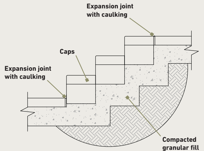
Figure 5.9-1 | Stair Construction
