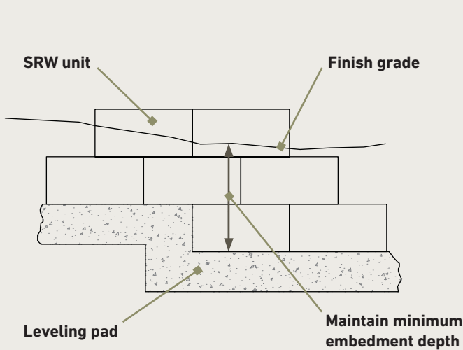
Figure 5.8-1 | Wall Step-Ups
