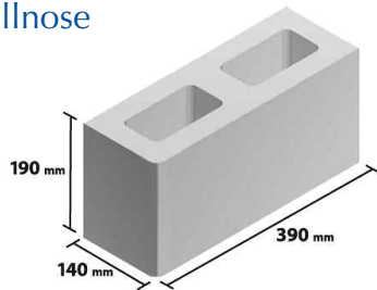
15 cm Double Bullnose
