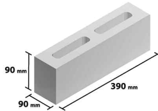
10 cm Half High
