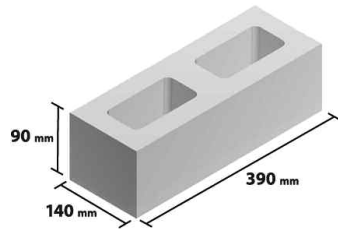
15 cm Half High
