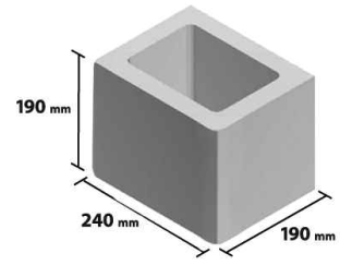
25 cm Double Bullnose Half
