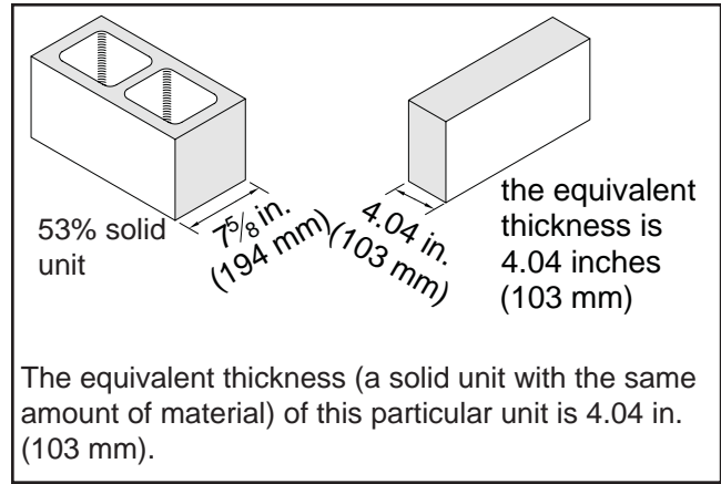
Figure 1—Equivalent Thickness
